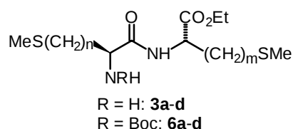
Scheme 1 Metal catalyzed Michael reactions of donor 1 with acceptor 2 ; in situ -formation of complexes of chiral ligands 3a–d with metal salts 4a–m
